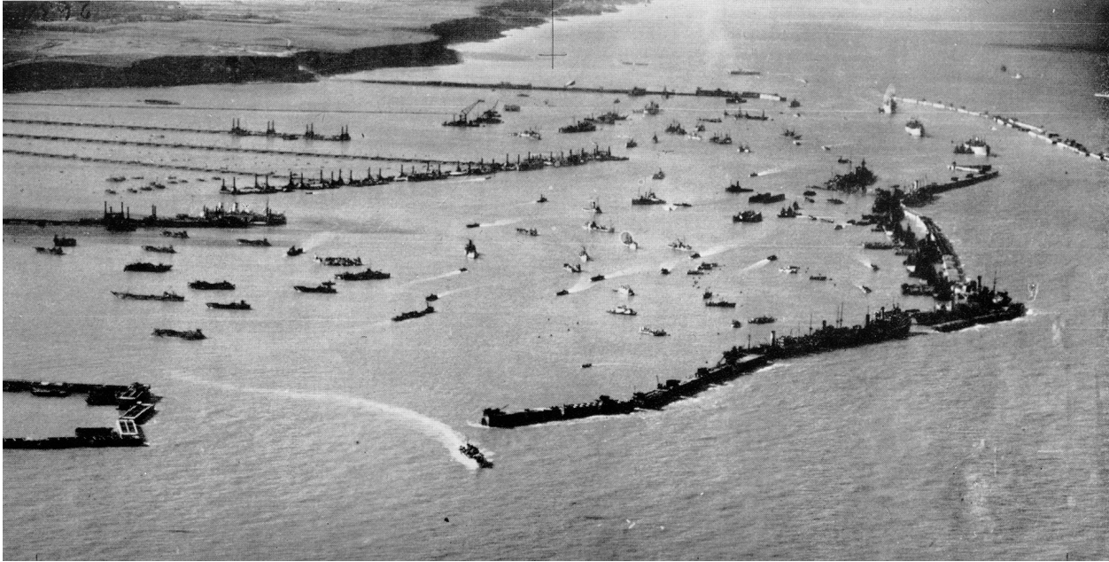
Figure I-3-14. Aerial photograph of the Mulberry “B” Harbor at Arromanches, France, June 1944 (from Institution of Civil Engineers, London, England, 1948, p. 242)
